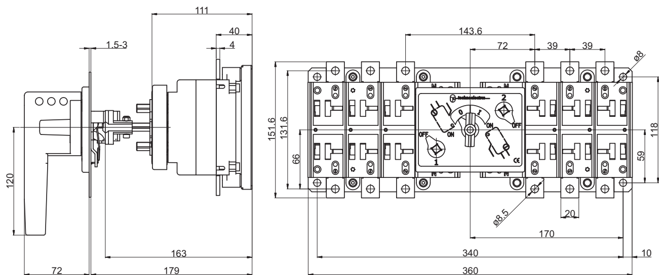
TS056P
