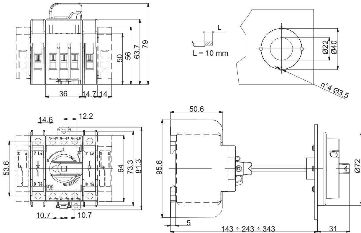
TS015M
