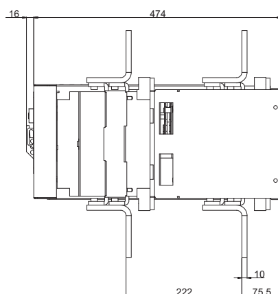
CS6MS 2000 A FN
