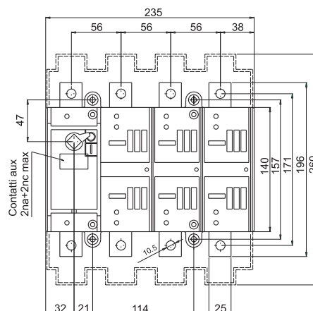
VC3P 315 ÷ 500 A
