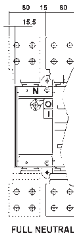
FULL NEUTRAL
