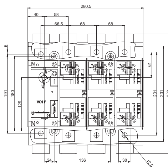
VC4F 315 ÷ 400 A
