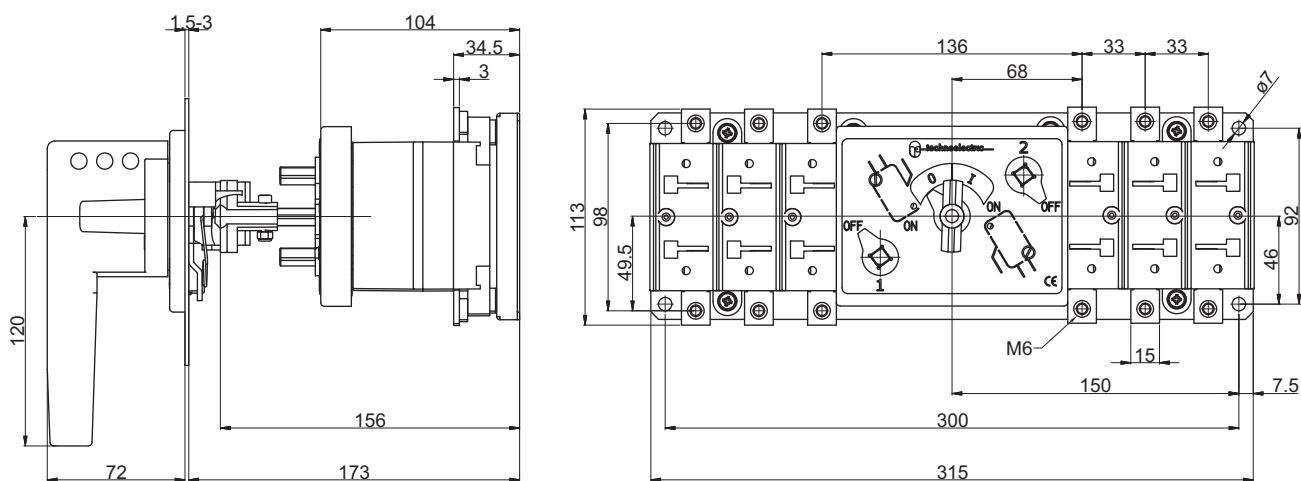
TS046P
