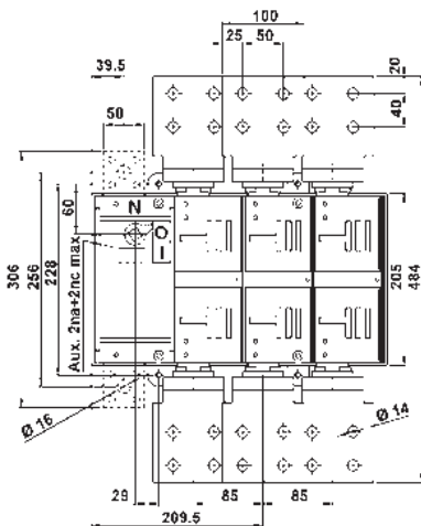
NEUTRAL 2000A
