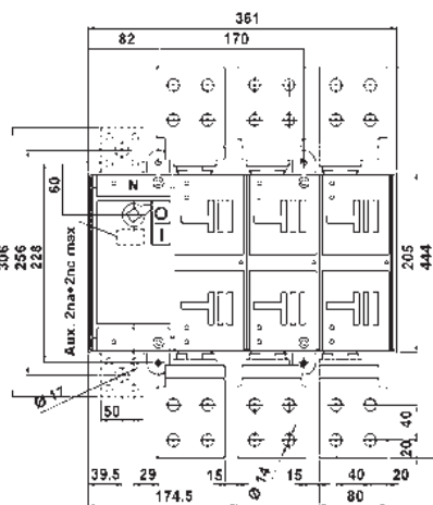
FULL NEUTRAL
