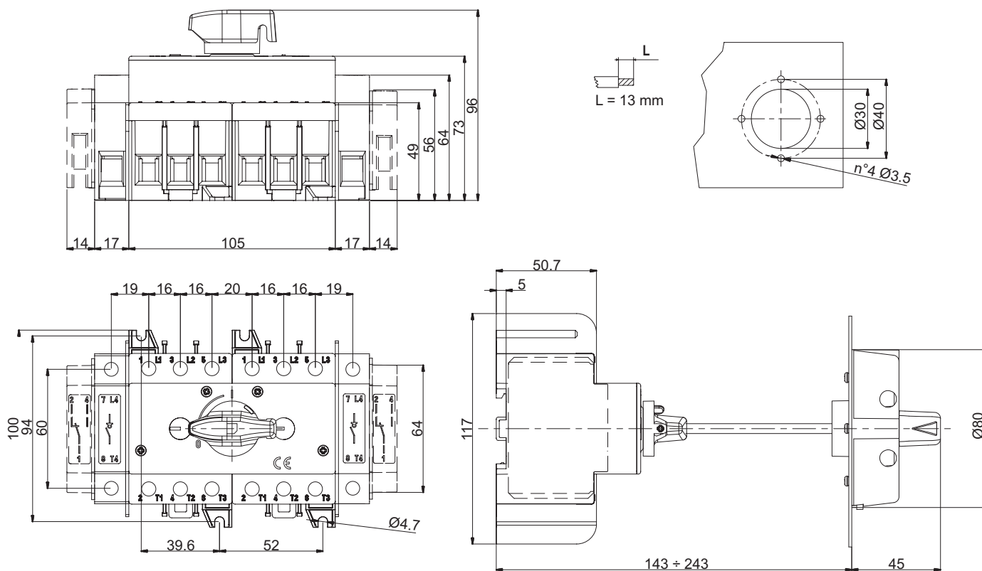
TS028M
