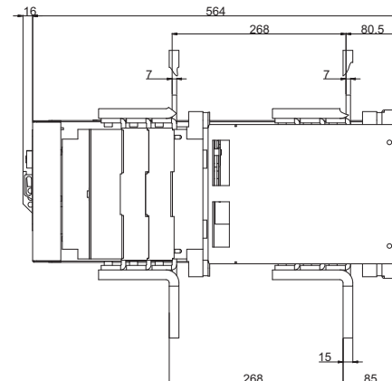
CS6 2500 A N 1250 A
