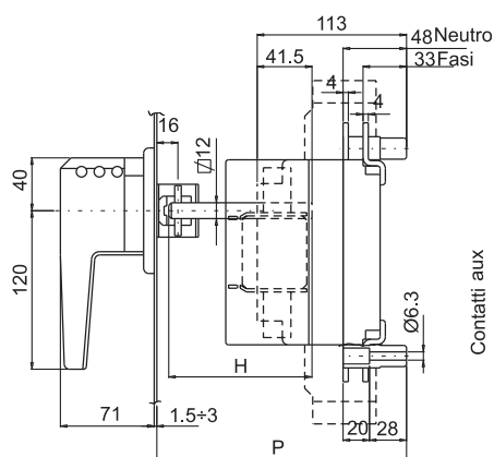
VC3F
