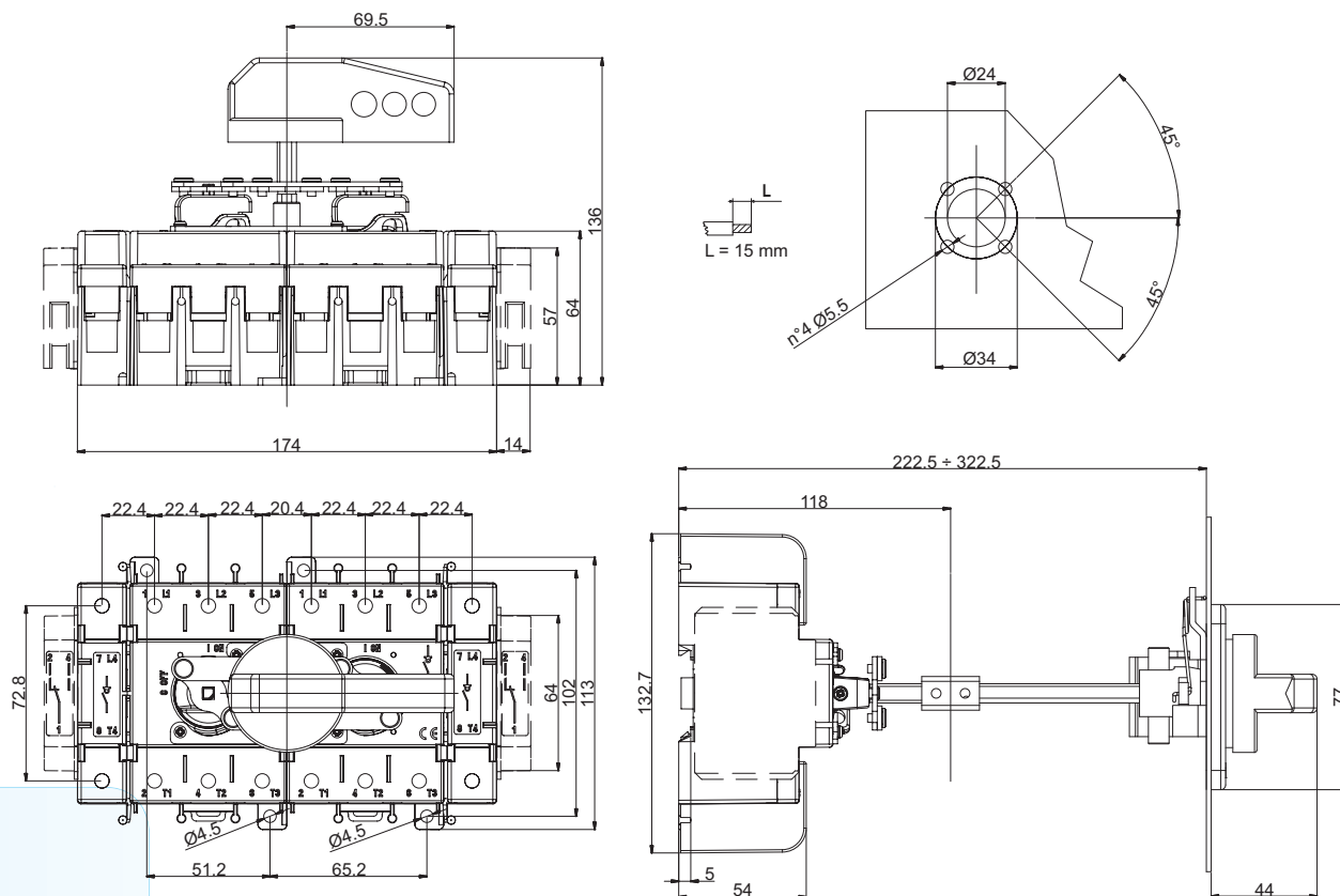
TS038M
