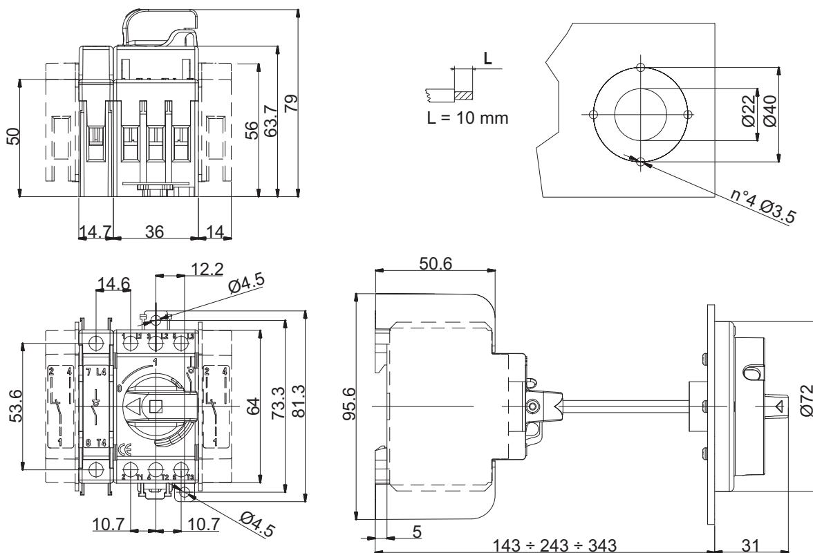
TS014M
