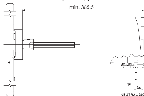
NEUTRAL 2000A
