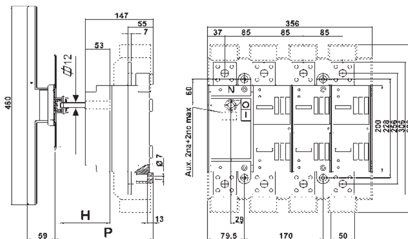
VC5P
