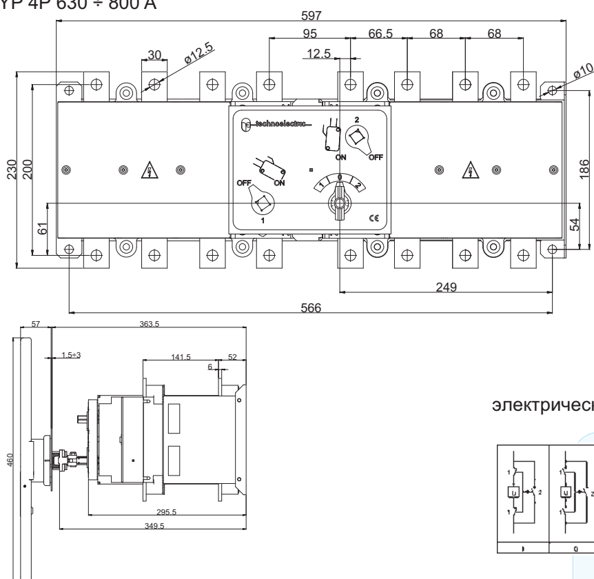
BY 4P 630 ÷ 800 A
